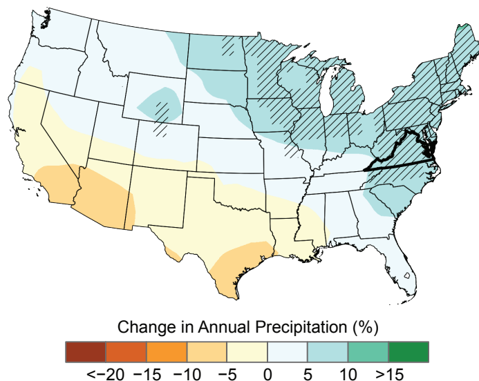
Figure 6: Projected change in annual precipitation (%) for the middle of the 21st century compared to the late 20th century under a higher emissions pathway. Hatching represents areas where the majority of climate models indicate a statistically significant change. Virginia is part of a large area of projected increases that includes all of the northeastern United States. Source: CICS-NC, NOAA NCEI, and NEMAC.
