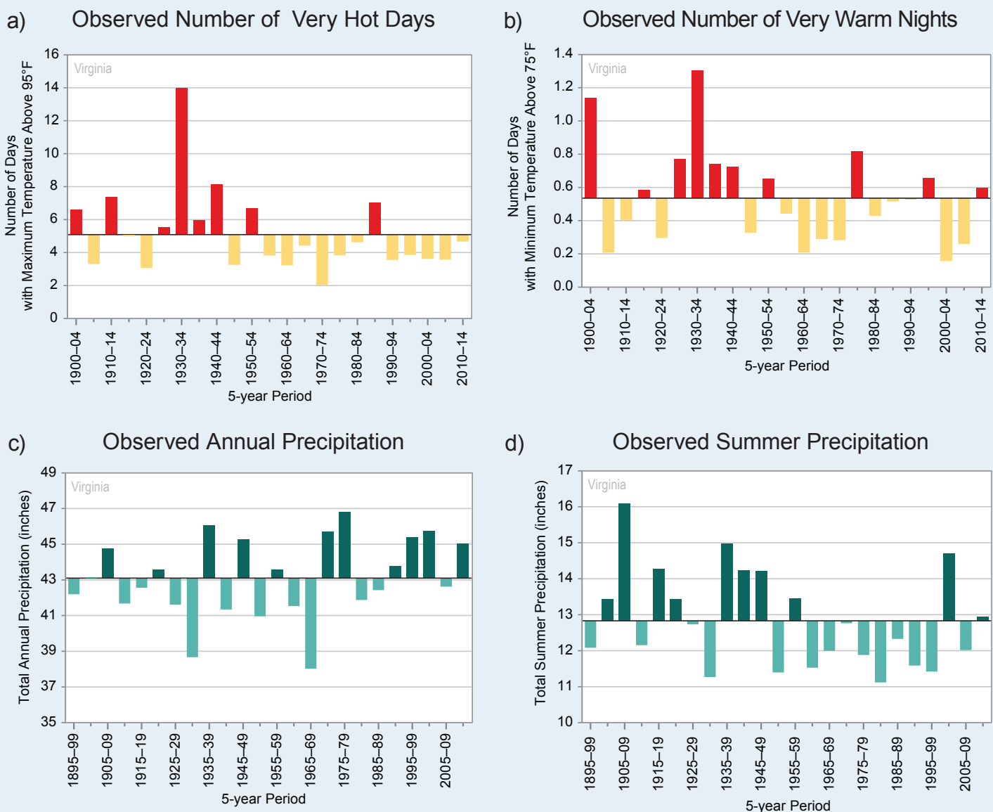
Figure 2: The observed (a) number of very hot days (maximum temperature above 95°F), (b) number of very warm nights (minimum temperature above 75°F), (c) annual precipitation, and (d) summer precipitation, averaged over 5-year periods. The values in Figures 2a and 2b are from nine long-term reporting stations. The values in Figures 2c and 2d are from NCEI's version 2 climate division dataset. The dark horizontal lines represent the long-term average. The number of very hot days and very warm nights peaked in the 1930s and has subsequently remained near to below the long-term average. There is no overall trend in average annual precipitation; summer precipitation has been below or near average during the most recent decade (2005–2014). Source: CICS-NC and NOAA NCEI.
