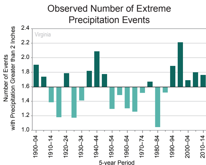
Figure 5: The observed number of extreme precipitation events (precipitation amounts greater than 2 inches) for 1900–2014, averaged over 5-year periods; these values are averages from 10 long-term reporting stations. The number of events is highly variable but exhibits a long-term upward trend. The 5-year period between 1995 and 1999 surpassed a 1940s record. The dark horizontal line is the long-term average (1900–2014) of 1.6 days per year. Source: CICS-NC and NOAA NCEI.
